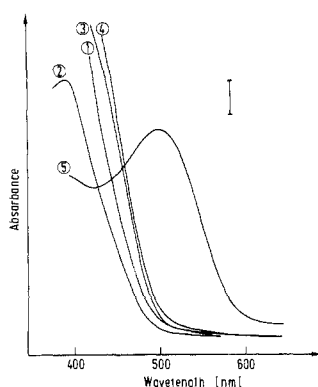
Figure 4. Incubation of opsin (15 nmol in 1 mL of 50 mM phosphate buffer, pH 7.0) with the 13-cis (6 nmol, curve 1), 9,13-dicis (40 nmol, curve 2), 9-cis (86 nmol, curve 3), and all-trans isomer (9 nmol, curve 4) of retinal 4. Curve 5 shows the regeneration of opsin upon addition of 40 nmol of 11-cis-retinal (1) to the incubation mixture. Full scales were 0.2 for curves 1 and 4, 2.0 for curves 2 and 3, and 1.0 for curve 5. The bar corresponds to 0.1 OD units at a full scale of 1.0.
