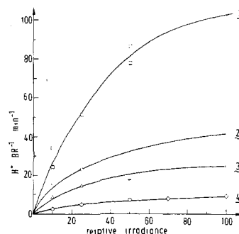
Figure 6. Light-induced proton translocation in cell vesicles containing reconstituted BR's. The BR's were reconstituted with retinal (1) (yielding 13.2 nmol of BR, curve 1, 530-nm cutoff filter), with acetylenic retinal 2 (19 nmol, curve 2, 480-nm cutoff filter), with acetylenic retinal 3 (11 nmol, curve 3, 480-nm cutoff filter), and with acetylenic retinal 4 (6.2 nmol, curve 4, 455-nm cutoff filter). Illumination was with light from a 150W slide projector bulb filtered through the respective cutoff filters. For details see ref 26.
