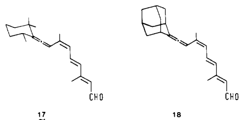
Figure 7. Structures of allenic retinals 17 and 18 mentioned in the text. 36,37
