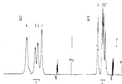
Figure 3. Analytical HPLC traces of the illuminated all- trans isomer of acetylenic retinal 2 in isopropyl alcohol, detected at 360 nm. (a) After 15 s of illumination. (b) After 5 min of illumination. 1 = 13- cis , 2 = 9,13- dicis , 3 = 9- cis , and 4 = all- trans isomer. The vertical bar corresponds to 0.02 OD units. The polarity of the solvent increased slightly from the injection shown in (a) to that shown in (b), leading to a faster elution of all isomers. For conditions of illumination and of HPLC see Experimental Section. The identification of the isomers was performed by 400-MHz 1 H NMR (see Table I).
