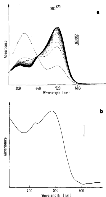
Figure 5. (a) Formation of a BR analogue containing the acetylenic retinal 3. To a 1-mL suspension of 5 nmol of AM at 10 °C, 3.5 nmol of the all-trans isomer of 3 was added (reference: 5 nmol of AM in 1 mL of water). Spectra were recorded at: 20 (spectrum with the lowest absorption at 520 nm), 40, 80, 120, 170, 220, 260, 310, 350, 390, 440, 490, 530, 580, 620, 660, 760, and 810 s (spectrum with the highest absorption at 520 nm). (b) Spectrum of a BR analogue containing the acetylenic retinal 4. Retinal-deficient cells were grown in the presence of 4. The spectrum was taken after the cells were lysed in water. The shoulder at 420 nm is due to contaminating cytochromes (soret band). The sample was measured in a 0.2-cm path length cuvette at a full scale of 2.0. The bar inserted corresponds to 0.2 OD units.
