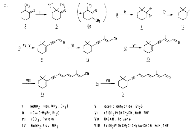
Figure 1. Structures of the all- trans isomers of retinal (1), 7,8-dehydroretinal (2), 5-desmethyl-7,8-dehydroretinal (3), and 1,1,5-tridesmethyl-7,8-dehydroretinal (4). The formula of retinal was superimposed (dashed) on the formulas of 3 and 4 to demonstrate the changes in shape upon the introduction of the acetylenic bond. Two possible arrangements of the acetylenic retinals result. Either the cyclohexane ring (demonstrated with compound 3) or the carbonyl end group (demonstrated with compound 4) are fixed in the same position as in retinal.
