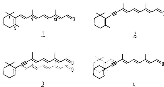
Figure 1. Structures of the all- trans isomers of retinal (1), 7,8-dehydroretinal (2), 5-desmethyl-7,8-dehydroretinal (3), and 1,1,5-tridesmethyl-7,8-dehydroretinal (4). The formula of retinal was superimposed (dashed) on the formulas of 3 and 4 to demonstrate the changes in shape upon the introduction of the acetylenic bond. Two possible arrangements of the acetylenic retinals result. Either the cyclohexane ring (demonstrated with compound 3) or the carbonyl end group (demonstrated with compound 4) are fixed in the same position as in retinal.
