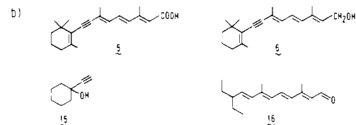
Figure 2. (a) Scheme of the synthesis of retinal 3. (b) Structures of compounds mentioned in the text.
