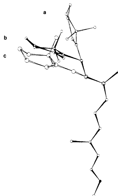
Figure 8. Superposition of the structure of allenic retinal 17 (a) on the structure of retinal 1 (b), which is shown in the 90° tilted conformation of ring and polyene side chain, and on the structure of acetylenic retinal 3 (c), also presented in the 90° tilted ring/side chain conformation. All compounds are shown in the 9- cis configuration.
